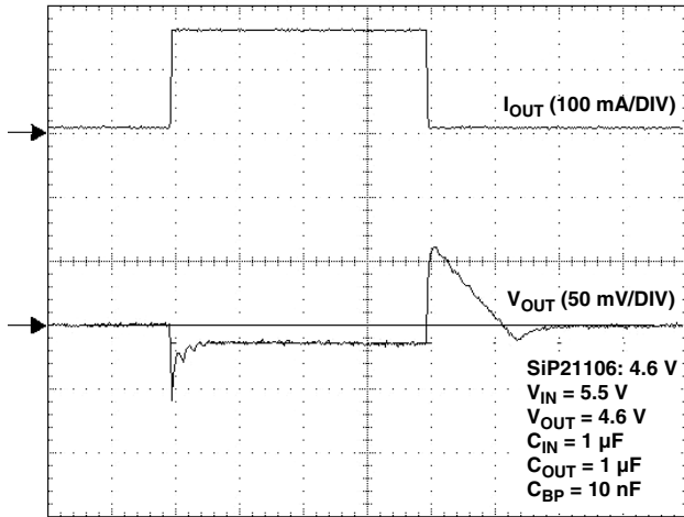
50 μs/DIV Load Transient Response
