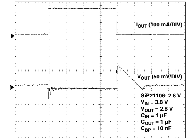
50 μs/DIV Load Transient Response
