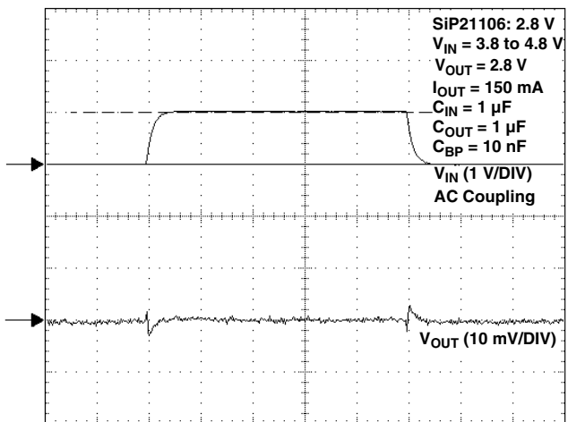
200 μs/DIV Line Transient Response
